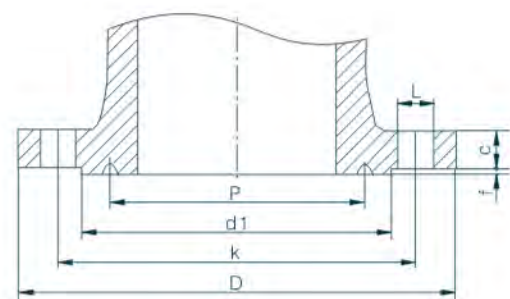
RTJ
