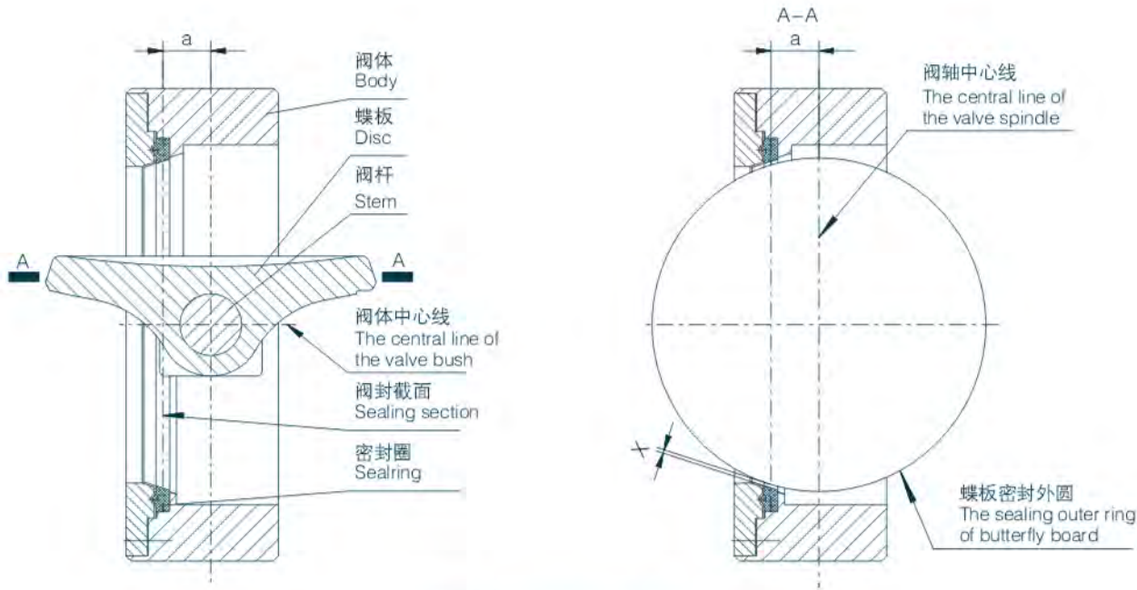
单偏心密封蝶阀密封副结构 The sealing structure of the single eccentric seal butterfly valve
