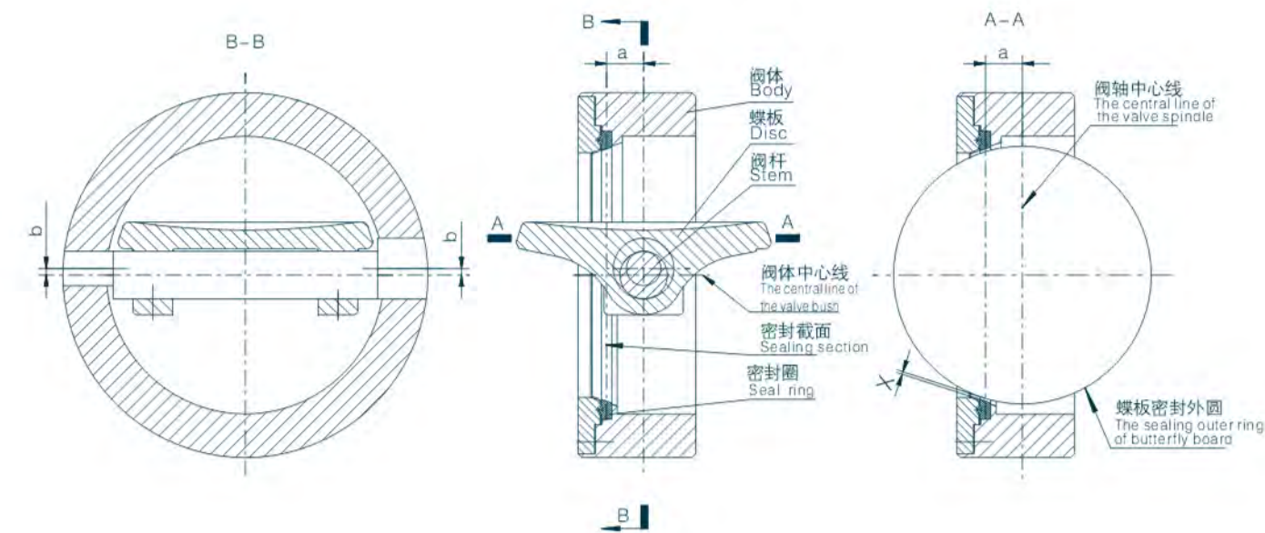
变偏心密封蝶阀密封副结构 The sealing structure of the various eccentric seal butterfly valve
